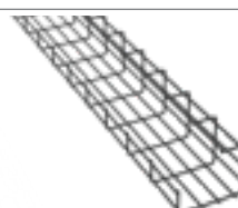
X-Tray 120x150 L=2300 mm | Draad Ø 5
